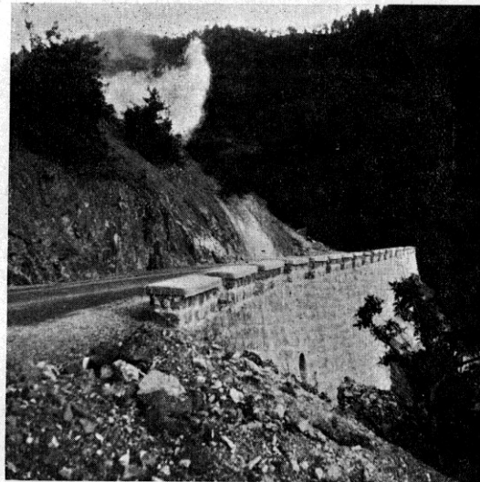
Fig. 7. Retaining Wall.
