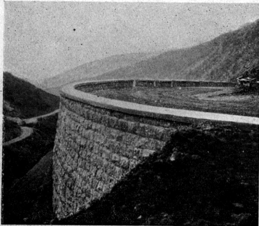
Fig. 5. A Bend of the Zigana Pass.
