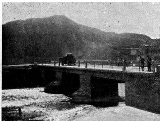
Fig. 18. New Deck on Old Piers.
