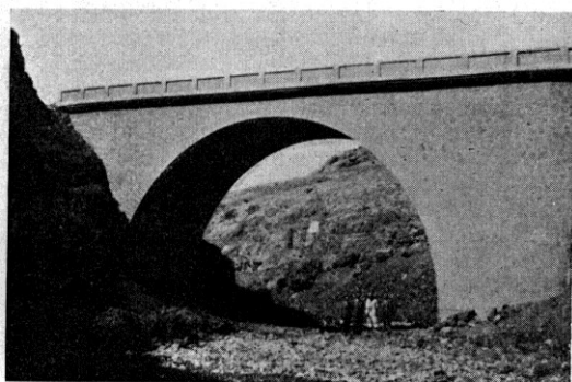
Fig. 16. Plain Concrete Arch Viaduct.
